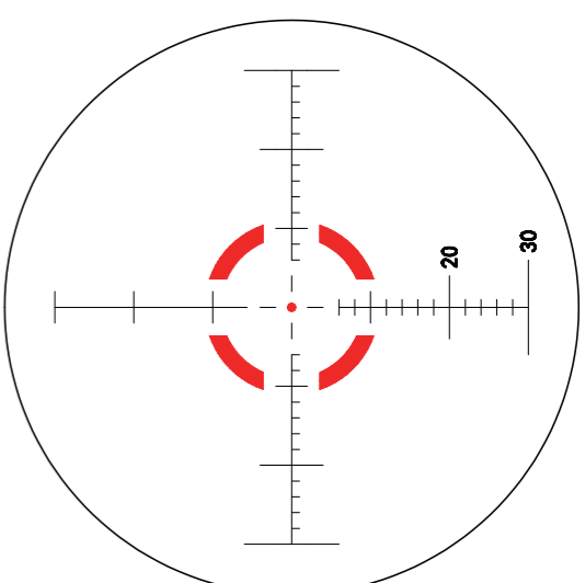
Etched Glass M-4RD Reticle
